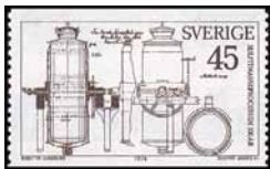
Drawing of First Industrial Digester A265
